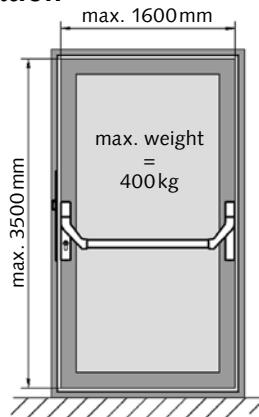
Single leaf - DIN left side
