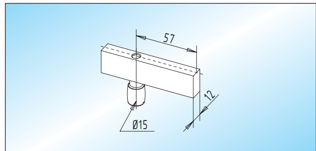
Top centre aluminium top centre with stainless steel pivot pin
