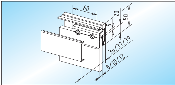
KR 50 - Clamping rail clamping rail with base profile, glass clamps and cover
