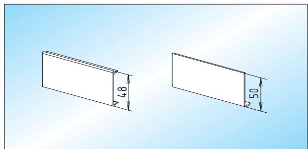
Cover aluminium cover / 48 mm to clip on base profile (only used one-side)
