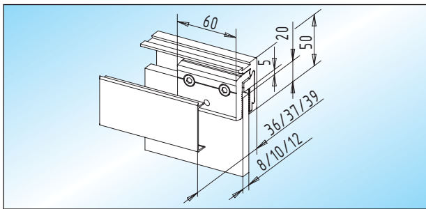
KR 50.1 - Clamping rail clamping rail with base profile, glass clamps with security pin and cover. Glass preparation: page 328
