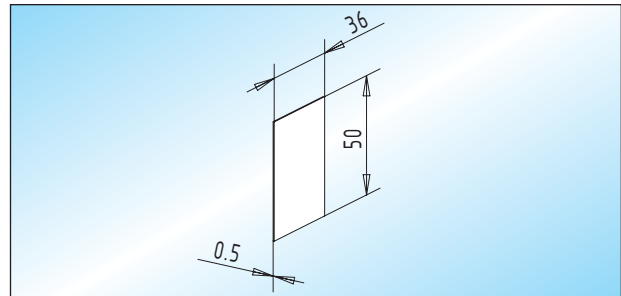
Endcap aluminium endcap, self adhesive
