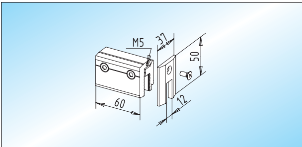
Endcap aluminium endcap and glass clamp
