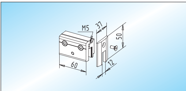
Endcap aluminium endcap and glass clamp with security pin Glass preparation: page 328
